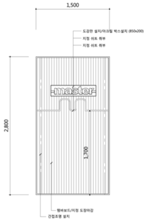
FRONT VIEW SCALE 1/30
